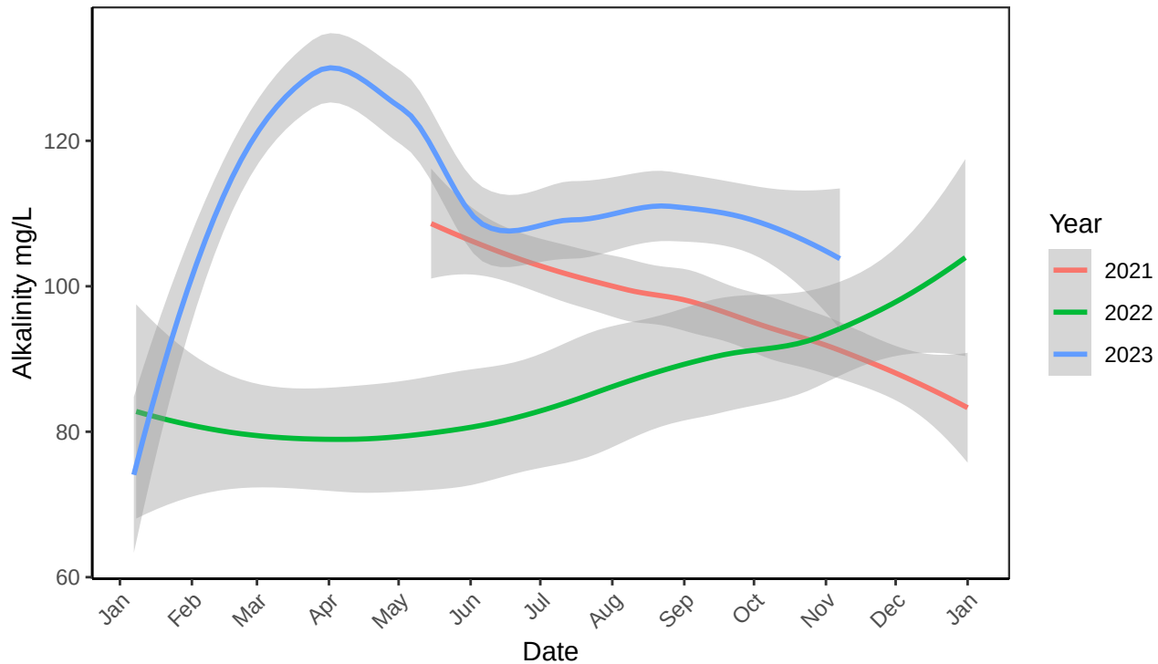
B2 Raceway 2 Alkalinity mg/L
